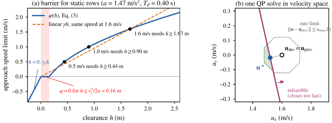
FIGURE 3. Mid-level safety filter with mission parameters. (a) \varphi(h) of Eq. (3) for static rows: zero below h = 0.16 \text{ m} , h \geq 1.67 \text{ m} needed at 1.6 \text{ m/s} ; a linear \gamma h permits approach where \varphi demands a stop. (b) One QP solve by the flight code for an illustrative case (cylinder 2.51 \text{ m} ahead): the closing speed drops from 1.56 to 1.48 \text{ m/s} .
