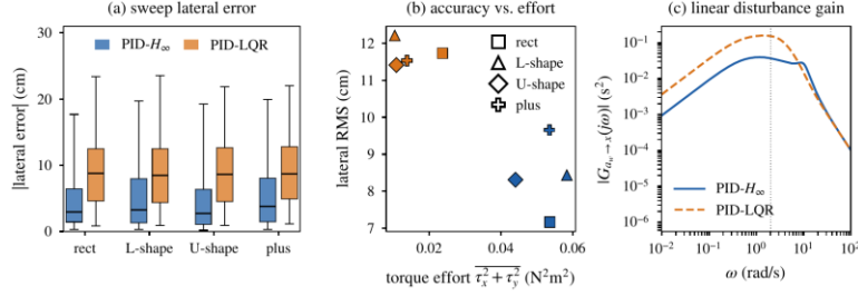
FIGURE 8. (a) Absolute lateral error in steady east–west sweeps (box: quartiles, whiskers: 5th–95th percentiles). (b) RMS lateral error against torque effort. (c) Disturbance-to-position gain of the linearised outer loop; dotted: wind-model corner frequency.
